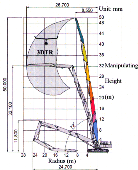
Fig. 2. A high-speed ground-based manipulation robot.
